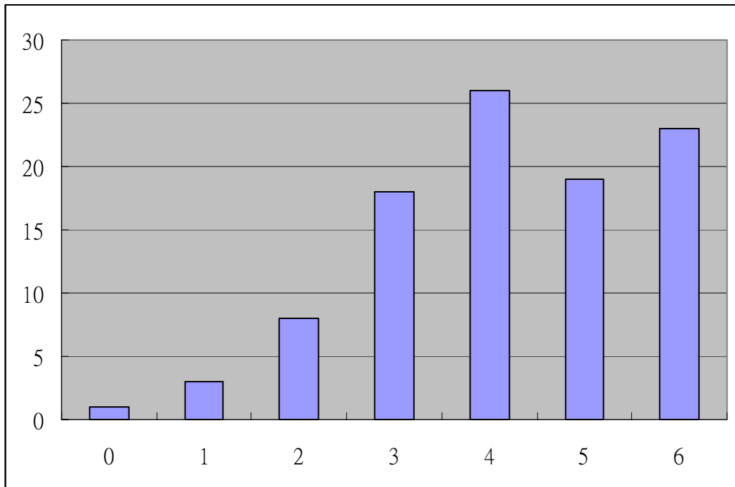
Quiz 8 Histogram
