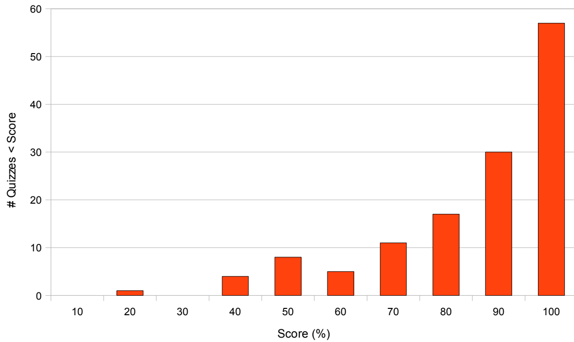
Quiz 5 Histogram
