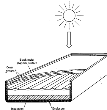
Figure 4.5 A cutaway view of a flat-plate solar collector with two cover glasses. A heat-transfer fluid is circulated through the tubular passages integrally formed into the metal absorber surface. (Not drawn to scale.)
