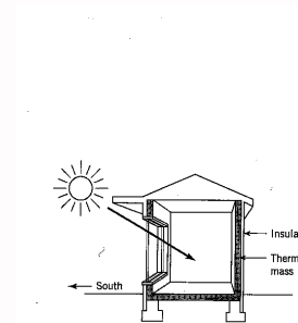
Figure 4.8 A home heated by the direct gain passive solar method. South-facing windows act as solar collectors. Sunlight enters the living space, is converted to heat at absorbing surfaces, and the heat is dispersed throughout the space and to the various enclosing surfaces and room contents. The windows can be covered at night with movable insulation to reduce heat loss. A massive masonry floor and back wall serve for heat storage and prevent overheating. The exterior overhang helps to prevent overheating in the summer. (Adapted from: J. Douglas Balcomb, Passive Solar Space Heating , Los Alamos National Laboratory, LA-UR-80-2555.)
