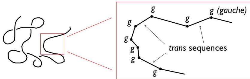
Figure 6.23: The polymer chain as a random coil.
