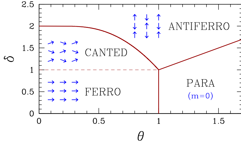
Figure 7.27: Mean field phase diagram for the model of eqn. 7.355 for the case \kappa = 1 .
