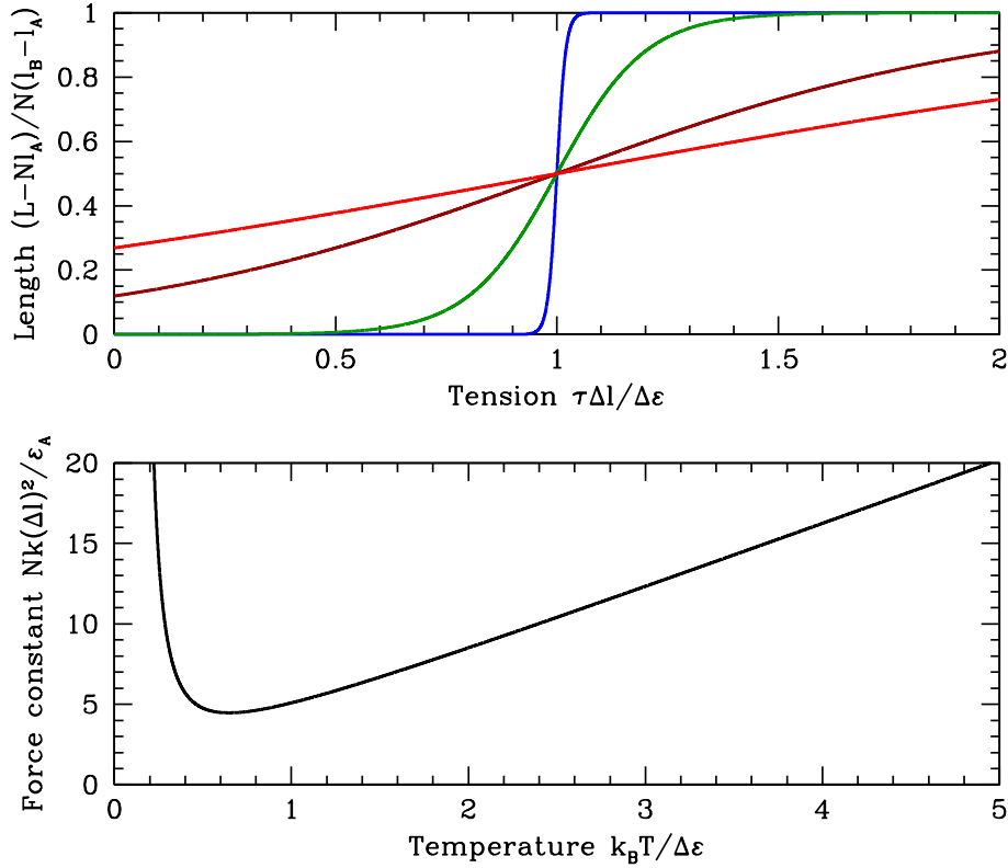
Figure 4.9: Upper panel: length L(\tau, T) for k_B T / \tilde{\epsilon} = 0.01 (blue), 0.1 (green), 0.5 (dark red), and 1.0 (red). Bottom panel: dimensionless force constant k/N(\Delta l)^2 versus temperature.
