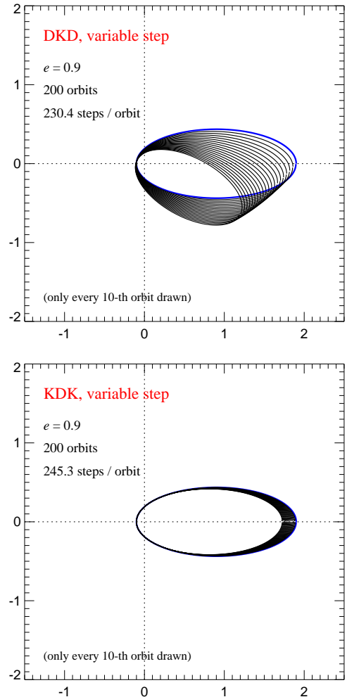
Figure 5. A Kepler problem of high eccentricity integrated with leapfrog schemes using a variable timestep from step to step, based on the \Delta t \propto 1/\sqrt{|a|} criterion commonly employed in cosmological simulations. As a result of the variable timesteps, the integration is no longer manifestly time reversible, and long term secular errors develop. Interestingly, the error in the KDK variant grows four times slower than in the DKD variant, despite being of equal computational cost.
