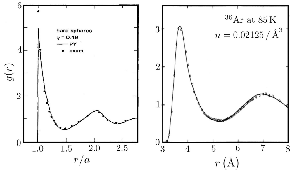
Figure 6.16: Pair distribution functions for hard spheres of diameter a at filling fraction \eta = \frac{\pi}{6} a^3 n = 0.49 (left) and for liquid Argon at T = 85 K (right). Molecular dynamics data for hard spheres (points) is compared with the result of the Percus-Yevick approximation (see below in §6.5.8). Reproduced (without permission) from J.-P. Hansen and I. R. McDonald, Theory of Simple Liquids , fig 5.5. Experimental data on liquid argon are from the neutron scattering work of J. L. Yarnell et al. , Phys. Rev. A 7 , 2130 (1973). The data (points) are compared with molecular dynamics calculations by Verlet (1967) for a Lennard-Jones fluid.
