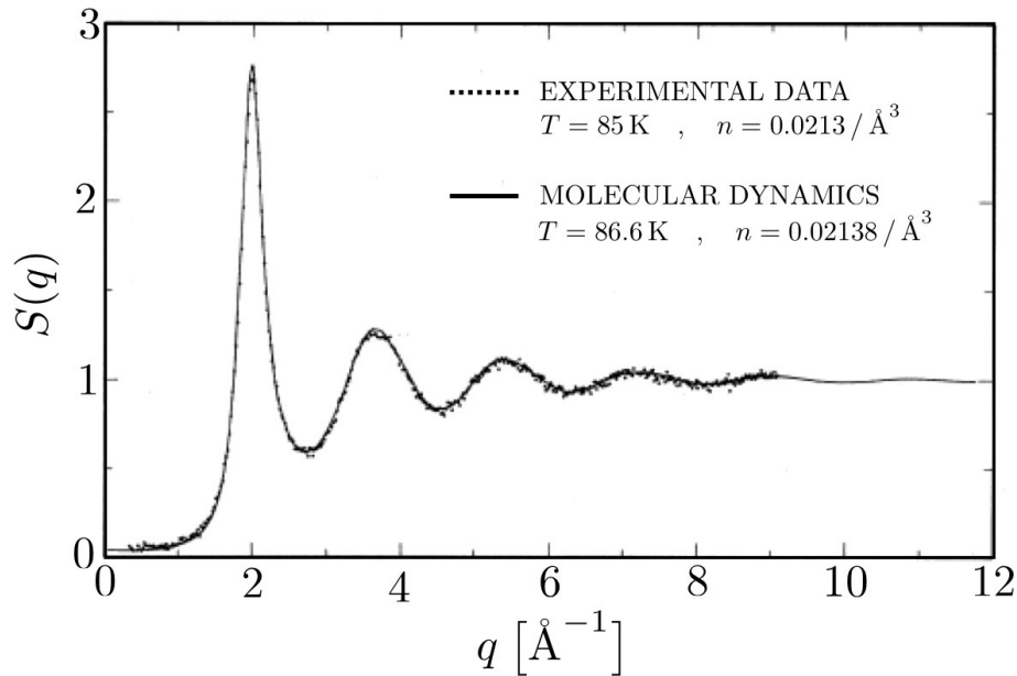
Figure 6.19: Comparison of the static structure factor as determined by neutron scattering work of J. L. Yarnell et al. , Phys. Rev. A 7 , 2130 (1973) with molecular dynamics calculations by Verlet (1967) for a Lennard-Jones fluid.
