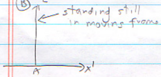
t' moving frame
