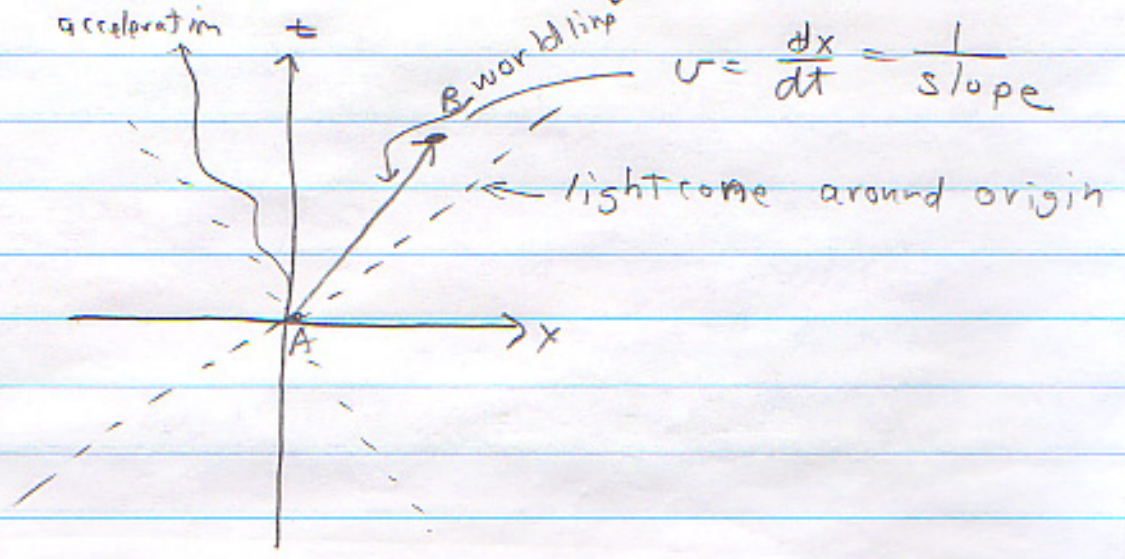
Figure: Space time diagram
