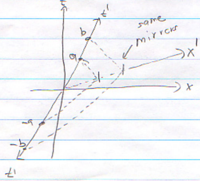
lab frame
