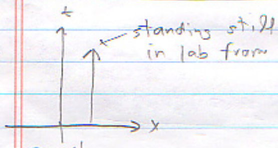
lab frame
