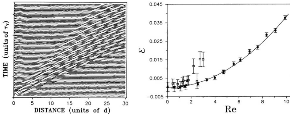
Fig. 37. The growth of a perturbation in the convectively unstable region of the phase diagram for Re=6 and \varepsilon=0.0477 ( \varepsilon - \varepsilon_c(Re) \approx 0.032 ) in the experiments by Tsameret and Steinberg [405] on Taylor-Couette flow with through flow. The pulse was generated by a sudden movement of the inlet boundary back and forth. Times are measured in units of the vertical diffusion time \tau_v ( =d^2/\nu with \nu the kinematic viscosity of the fluid) and the distance along the axis is measured in units of the gap spacing d . (b) The threshold to the convective instability \varepsilon_c(Re) as a function of Reynolds number Re in similar experiments by Tsameret and Steinberg [405]. The solid line marks the threshold according to a full theoretical stability calculation, and the solid circles the threshold values determined experimentally by tracing the evolution of a pulse generated near the inlet. The open squares are data obtained by extrapolation from a fit to the CGL equation down from higher \varepsilon values. At small enough values of Re , these agree to within experimental error.
