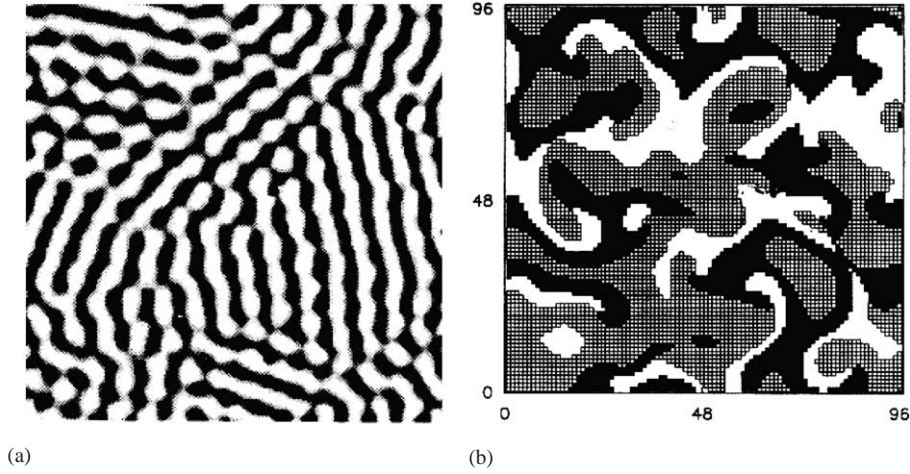
Fig. 28. (a) Snapshot of a convection pattern in a rotating Rayleigh–Bénard cell in the Kupperts–Lorz unstable regime, made with the shadowgraph technique. One identifies domains with essentially three orientations of rolls. From Bodenschatz et al. [51]. (b) A snapshot of the spatial pattern in the statistically steady state in simulations of Tu and Cross [407] of Eq. (116) with g_+ = 2 and g_- = 0.5 . The dark, grey and light regions represent the domains occupied by A_1 , A_2 and A_3 , respectively. The occupancy is determined by which one of the three amplitudes is largest.
