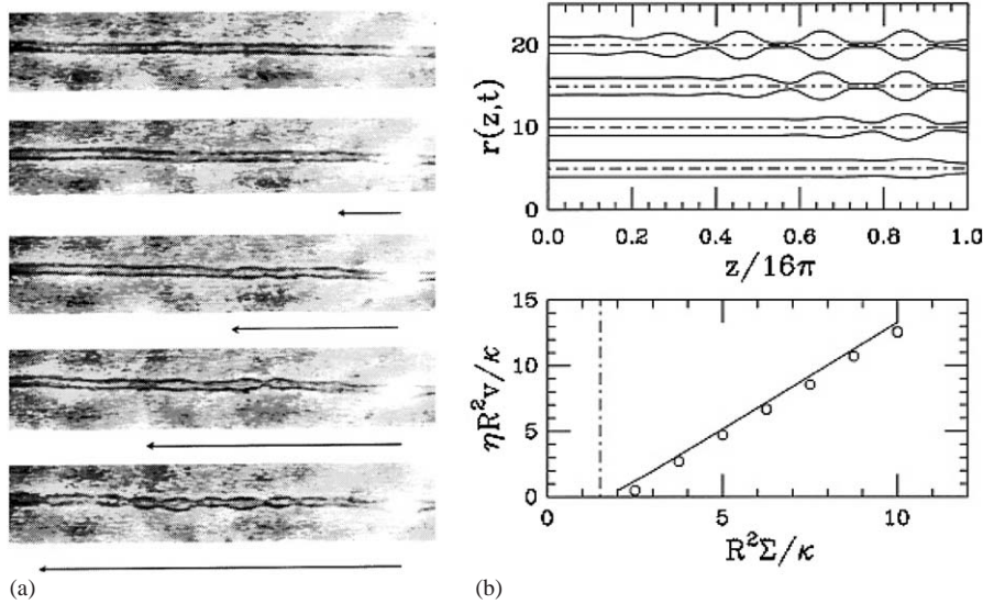
Fig. 25. (a) Photographs showing the pearly front along a tubular membrane formed by lipid bilayers in the experiments of Bar-Ziv et al. [26,27], as it propagates out from the bright laser spot on the right. In this experiment the dimensionless control parameter \varepsilon = (\Sigma - \Sigma_c) / \Sigma_c = 6.5 . From top to bottom the times are 0.14, 0.68, 0.86, 1.04 and 1.22 s after the laser was turned on. The arrow indicates the leading edge as it was determined by the authors. The height of each photographs corresponds to a distance of about 10 \mu\text{m} . (b) Results by Powers and Goldstein [356] for the simplified model (115) for the pearly instability. The top panel shows four snapshots of the pearly obtained from numerical simulation of the model. The higher snapshots are obtained at later times, so the front is traveling to the left. Bottom panel: dimensionless front velocity as a function of the ratio of surface tension and bending modulus. The solid line denotes the pulled front velocity v^* , the dots the data obtained in the numerical simulations. Note that the data points lie slightly below the curve for v^* . Undoubtedly, this is due to the slow convergence of the front speed to the asymptotic speed v^* .
