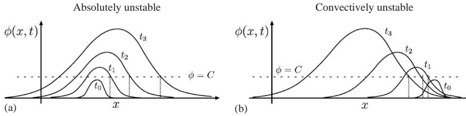
Fig. 7. Illustration of the distinction between an absolute instability and a convective instability, according to the linearized dynamics. In the first case, sketched on the left in (a), the perturbation about the unstable state grows for sufficiently long times at any position x . In the convectively unstable case sketched on the right in (b), the perturbation grows but is at the same time advected away so fast that it eventually dies at any fixed position x . Note that as a result of it, the point on the right where \phi reaches the level line \phi = C retracts to the left. The transition from convective to absolute instability occurs when this point does not move for long times, i.e. when the left spreading velocity v_L^* equals zero [49,62,204,205,264]. Note that the distinction between absolutely and convectively unstable depends on the frame of reference. The case sketched on the left which is absolutely unstable in the x frame is convectively unstable in a frame moving with a sufficiently large speed to the right, while the case sketched on the right in the x -frame becomes absolutely unstable in a frame moving with speed larger than v^* to the left.
