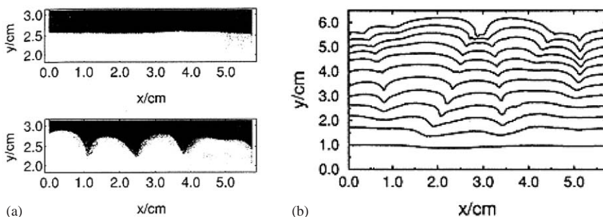
Fig. 43. (a) Front images in the experiments by Tóth and Horváth [398]. The upper image corresponds to the regime where the front is stable, while the lower one to the regime where the effective hydrogen diffusion coefficient is so small that the planar interface is unstable. The fronts are advancing upward. (b) Traces of the front positions in these experiments at time intervals of 120 min in the regime corresponding to the lower image of (a). The dynamics of the interfaces in this regime is very similar to that found in the Kuramoto–Sivashinsky equation, the generic lowest order equation just above threshold of a long-wavelength interface instability.
