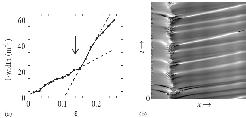
Fig. 42. (a) Dependence of the inverse of the average width of a source on the reduced control parameter \epsilon which measures the distance from the threshold at which traveling waves appear in the heated wire experiment of Pastur et al. [335,336]. The value of \epsilon_{\text{ca}} which was obtained independently from measurements of the group velocity s_0 , the correlation length \xi_0 and the time scale \tau_0 , is indicated by an arrow. At this point, a crossover in the inverse source width as a function of \epsilon is observed in the same way as in the numerical simulations, see Fig. 41(a). (b) Space–time diagram of the local wave number of a source in the experiments for \epsilon = 0.11 , i.e., in the incoherent source regime. The extent of the x -axis is 42 cm, the total time is 10485 s.
