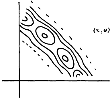
Fig. 1 Magnetic surface geometry for a single resonance.
