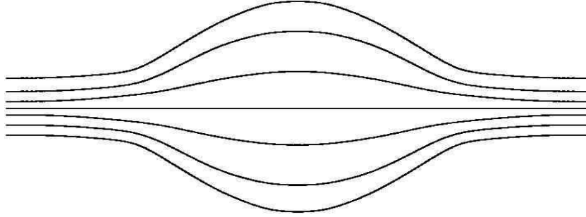
Figure 1.7: B field lines in a magnetic bottle.
