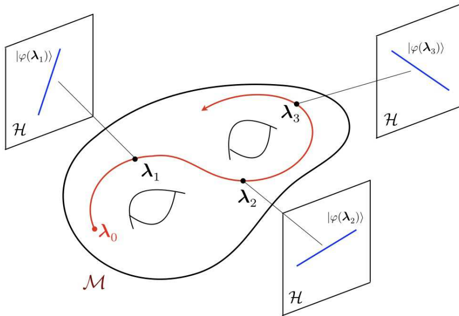
Figure 4.19: A Hermitian line bundle consists of a base space \mathcal{M} and a fiber |\varphi(\lambda)\rangle which twists as the point \lambda moves around the base space.
