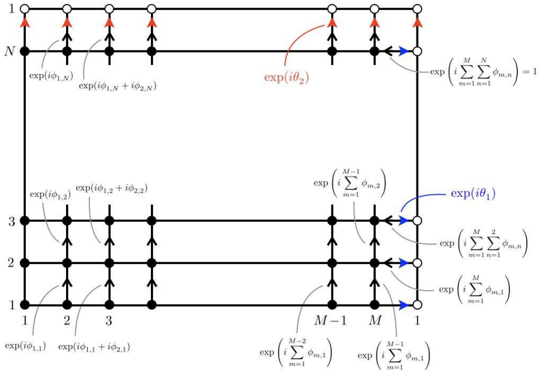
Figure 4.15: Lattice gauge field configuration for a general M \times N rectangular lattice with flux \phi_{m,n} in unit cell (m, n) and Bloch phases (\theta_1, \theta_2) .
