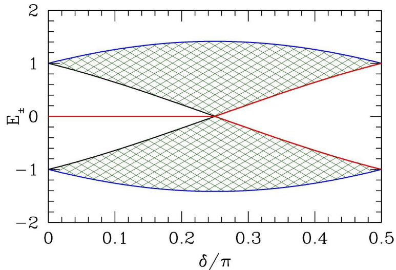
Figure 4.17: Spectrum of the SSH Hamiltonian on a finite chain with N_c \rightarrow \infty with t_1 = t \cos \delta and t_2 = t \sin \delta . The two E = 0 edge states exist provided |t_1| < |t_2| , i.e. |\delta| < \frac{\pi}{4} .
