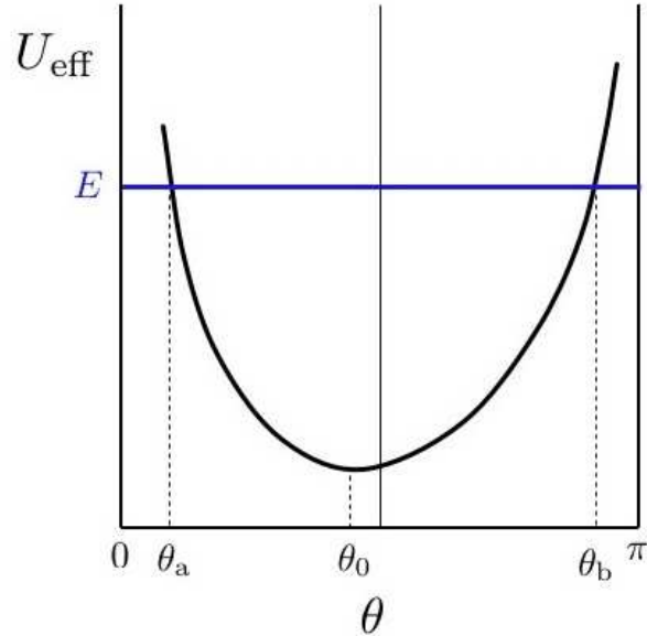
Figure 13.8: The effective potential of eq. 13.81.
