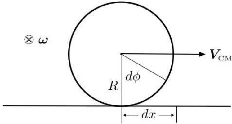
Figure 13.1: A wheel rolling to the right without slipping.
