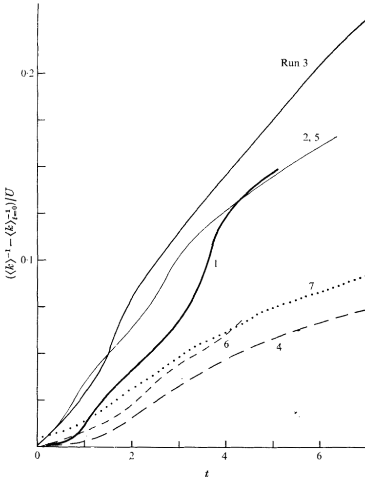
FIGURE 3. Experimental growth of the dominant scale of the eddy field with time. —, \beta = 0 ; ---, \dots , \beta > 0 . U_0 is the particle velocity at time t = 0 . Run numbers indicated.
