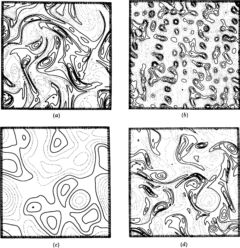
FIGURE 2. (a) Vorticity contours for a typical pure-turbulence run, \beta = 0 , using Fox & Orszag's spectral code. —, positive; - - - - -, negative. (b) Streamline field near the beginning of the free-evolution experiment (21st time step), \beta = 0 , run 2. Contour interval = 0.038. See table 1 for details. (c) Streamlines at t = 5.8 (725th time step), run 2. Contour interval = 0.1. (d) Vorticity contours at t = 5.8 , run 2. Contour interval = 1.3.
