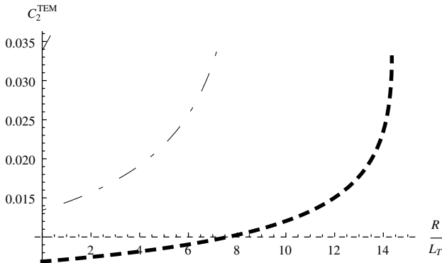
Figure 4. Plot of C_2^{\text{TEM}} as a function of R/L_{T_1} . The dashed line corresponds to R/L_n = 9 , the dash-dotted line to R/L_n = 6 and the solid line to R/L_n = 3 .
